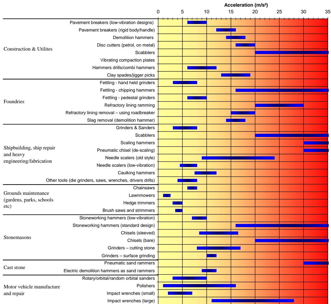
Figure 2 Examples of vibration magnitudes for common tools
