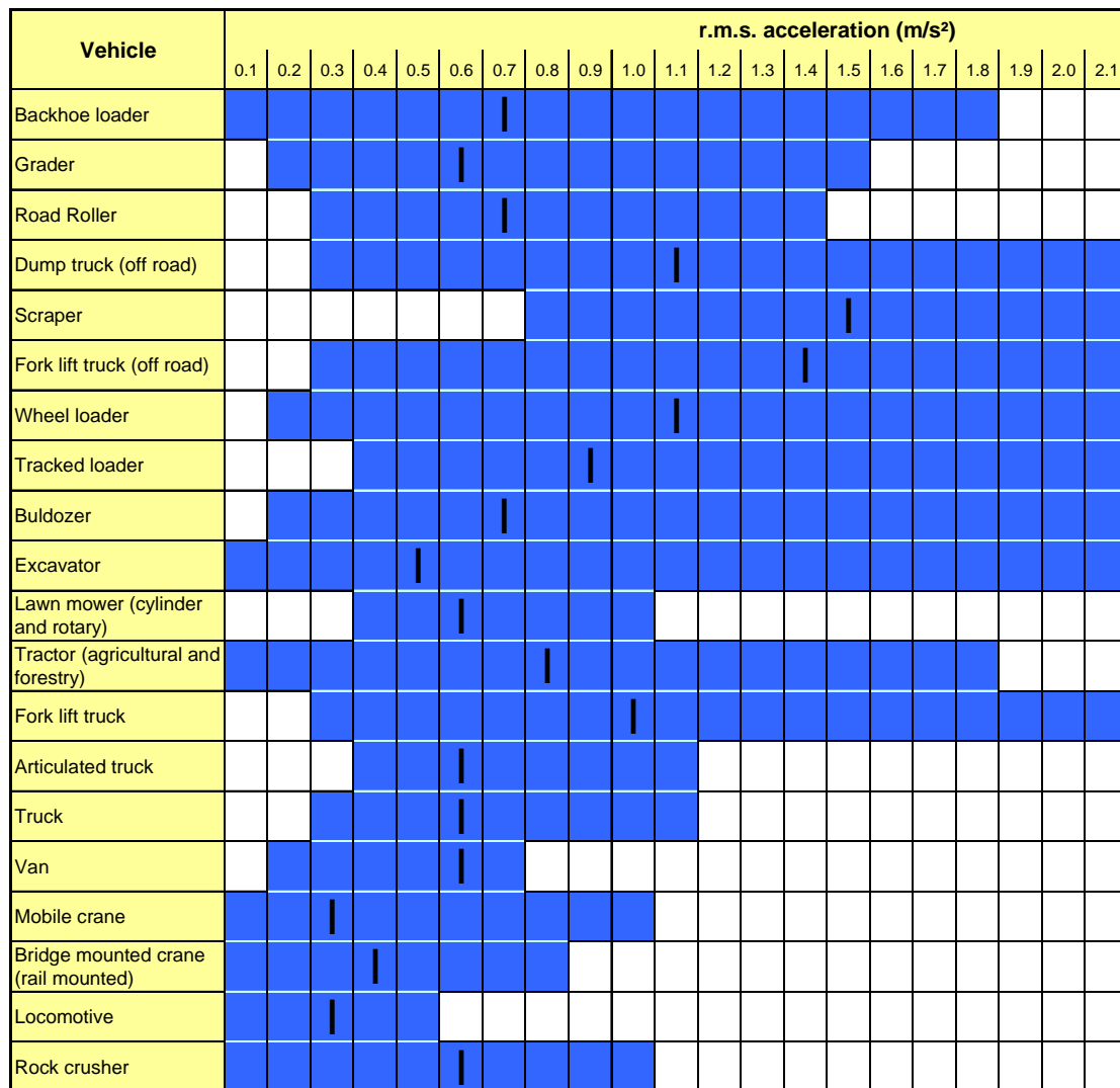
Figure 2 Examples of vibration magnitudes for common vehicles [Figure to be updated, based on data from INRS and others]
